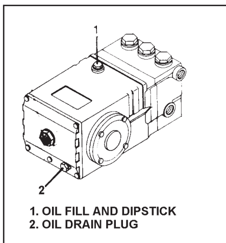
ILLUSTRATION #10 PUMP-REAR OIL GAUGE
