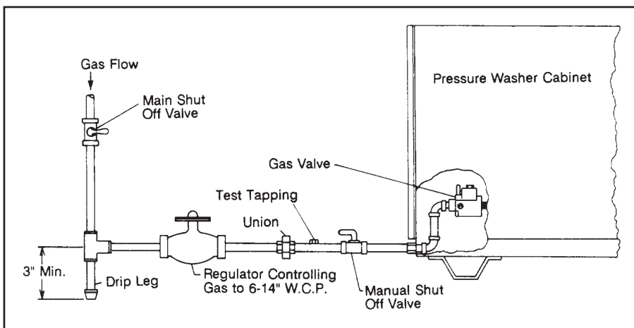
ILLUSTRATION #1 GAS SUPPLY PIPING
